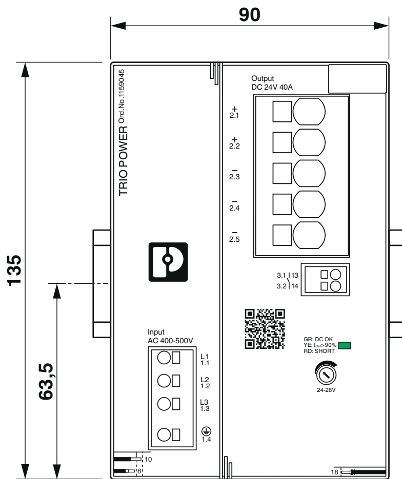
Dimensional drawing
